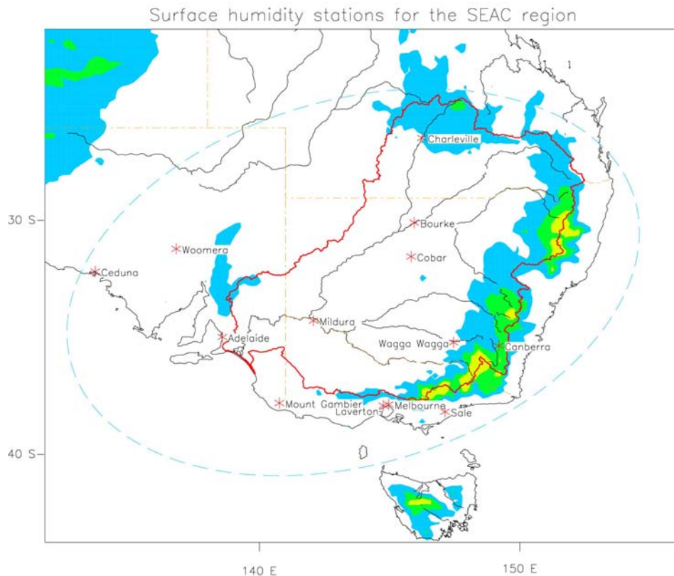
Figure A3-1: Locations of the surface humidity stations chosen for the SEACI program.
