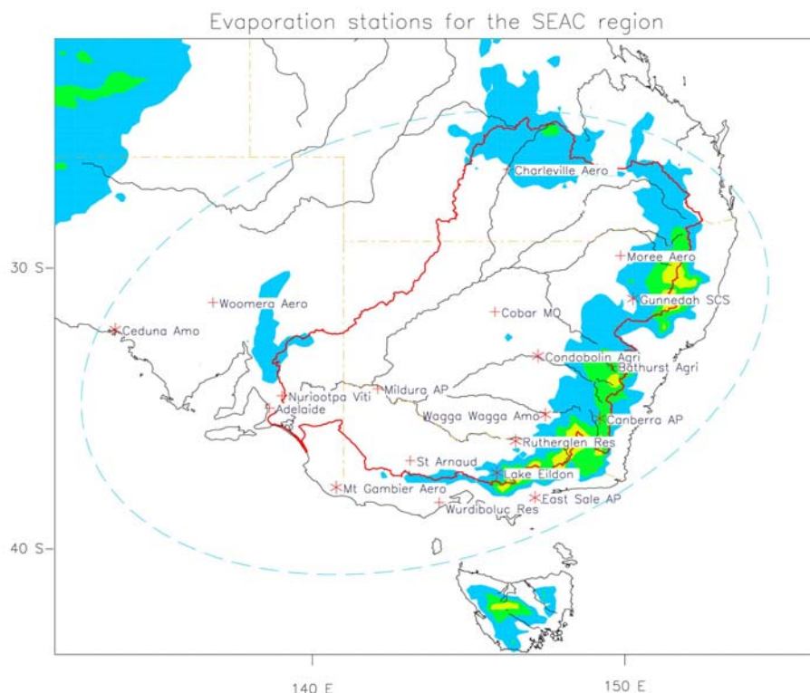
Figure A4-1: Locations of the pan-evaporation stations chosen for the SEACI program.
