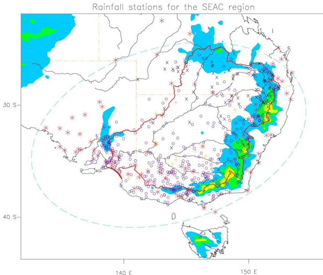
Figure A1-1: Locations of the rainfall stations chosen for the SEACI program.
