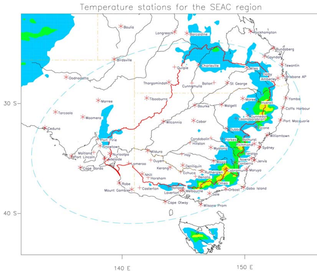
Figure A2-1: Locations of the temperature stations chosen for the SEACI program.
